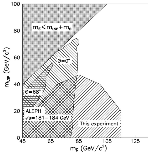
FIG. 2. The 95% C.L. exclusion contour in the (m_{\text{LSP}}, m_{\tilde{b}}) plane. Also shown are the results from the ALEPH experiment at LEP for minimal ( \theta=68^\circ ) and maximal ( \theta=0^\circ ) coupling [2].
